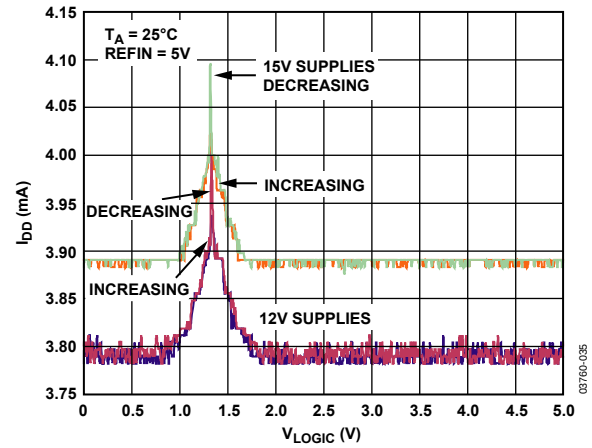
Figure 27. Supply Current vs. Logic Input Current for SCLK, \overline{\text{SYNC}} , SDIN, and \overline{\text{LDAC}} Increasing and Decreasing
