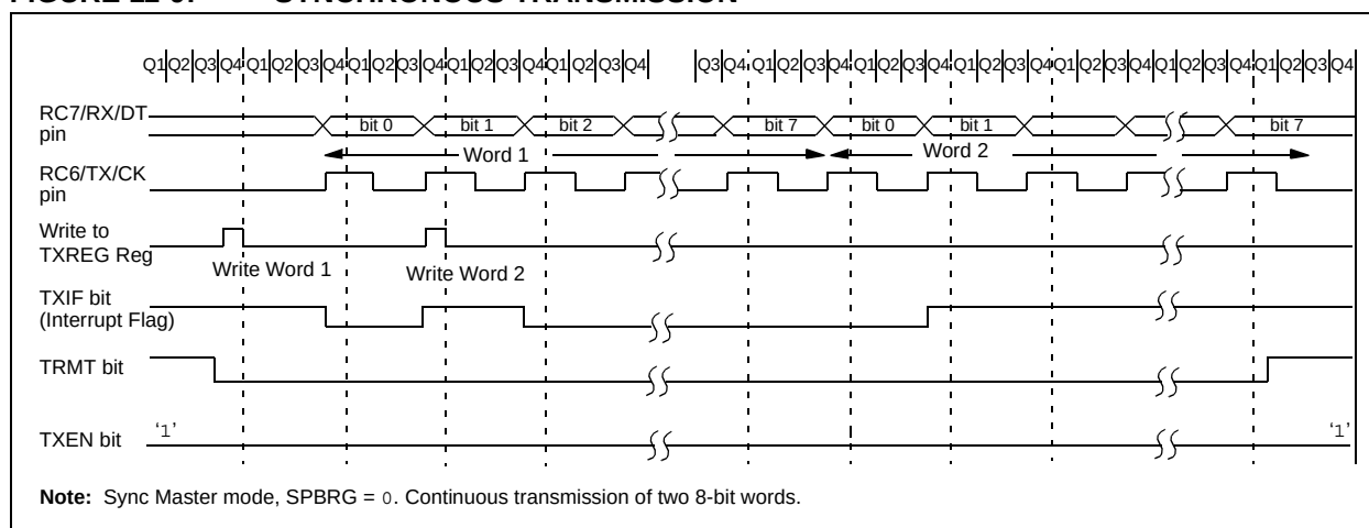
FIGURE 11-9: SYNCHRONOUS TRANSMISSION
