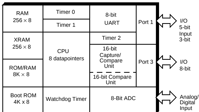
Figure 1 C868 Functional Units
