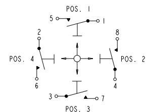
(C) SPST-NO 4 WAY SCHEMATIC
