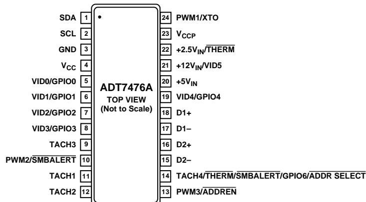
Figure 3. Pin Configuration
