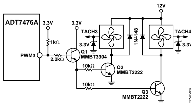
Figure 38. Interfacing Two Fans in Parallel to the PWM3 Output Using Low Cost NPN Transistors
