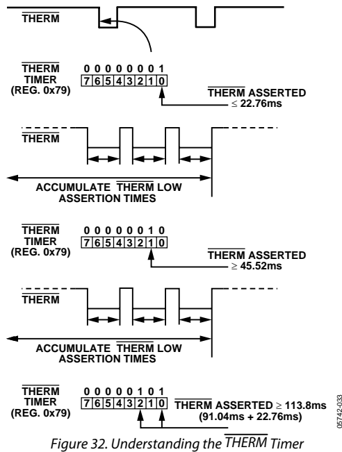
Figure 32. Understanding the \overline{\text{THERM}} Timer
