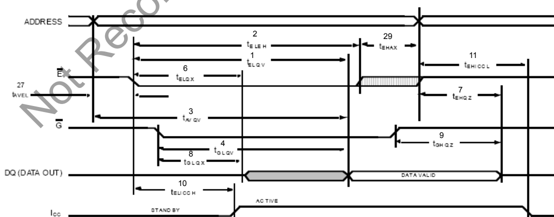
Figure 7. SRAM READ Cycle #2: \bar{E} and \bar{G} Controlled [3, 6]
