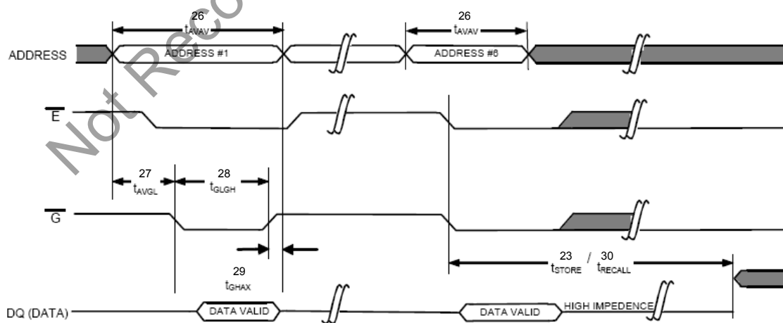
Figure 12. Software STORE/RECALL CYCLE: \overline{G} Controlled [13]
