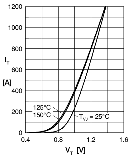
Fig. 1 Forward characteristics
