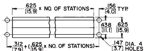
FIGURE A - PANEL CUTOUT FOR PLUNGER CLEARANCE ONLY
