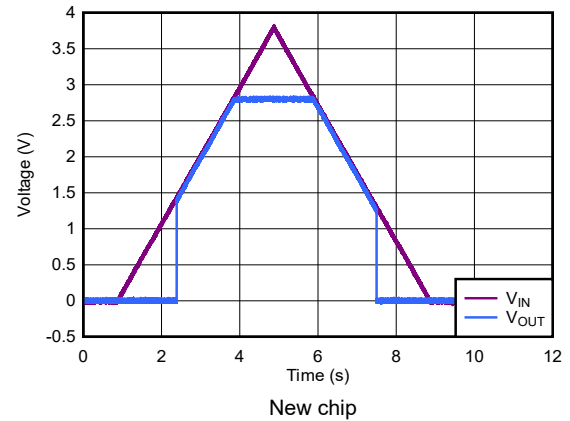
Figure 5-28. Power-Up and Power-Down
