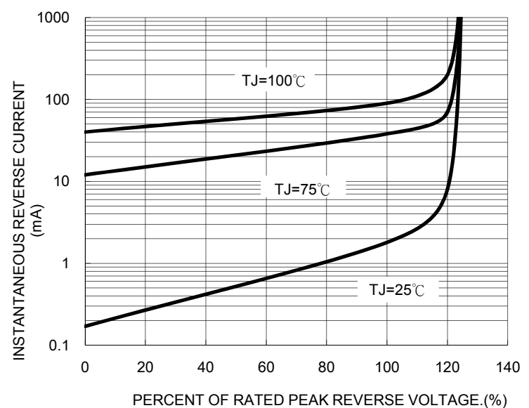
FIG. 4 TYPICAL RERVERSE CHARACTERISTICS
