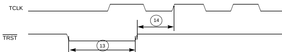
Figure 33-19. \overline{\text{TRST}} Timing
