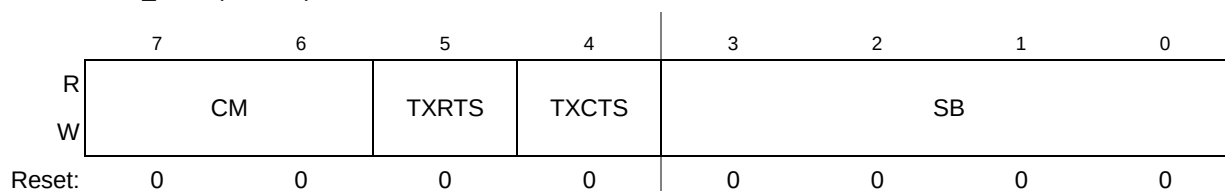
Figure 23-4. UART Mode Registers 2 (UMR2 n )
