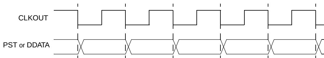
Figure 30-2. CLKOUT Timing
