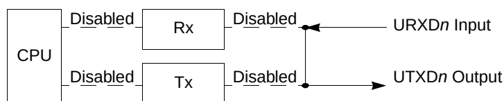
Figure 23-23. Remote Loopback
