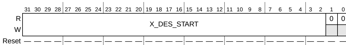
Figure 17-23. Transmit Buffer Descriptor Ring Start Register (ETSDR)
