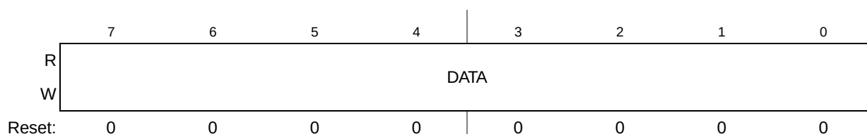
Figure 24-6. I 2 C Data I/O Register (I2DR)
