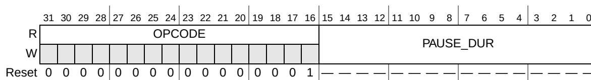
Figure 17-14. Opcode/Pause Duration Register (OPD)
