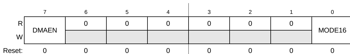
Figure 21-3. DTXMR n Registers
