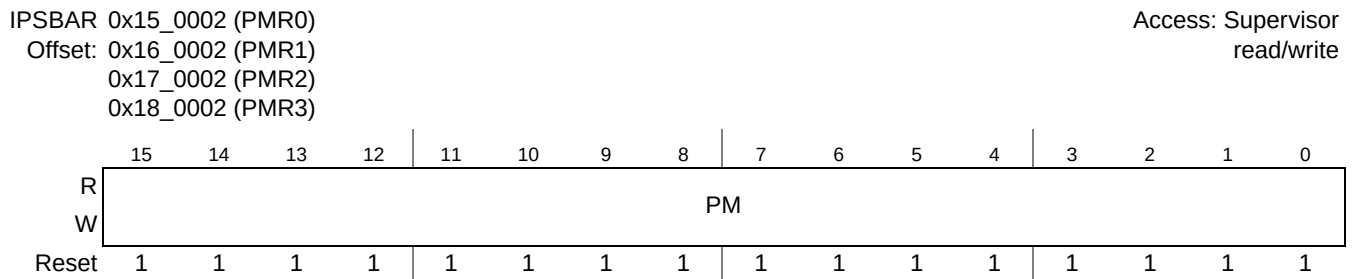
Figure 19-3. PIT Modulus Register (PMRn)
