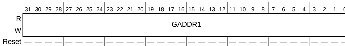
Figure 17-17. Descriptor Group Upper Address Register (GAUR)
