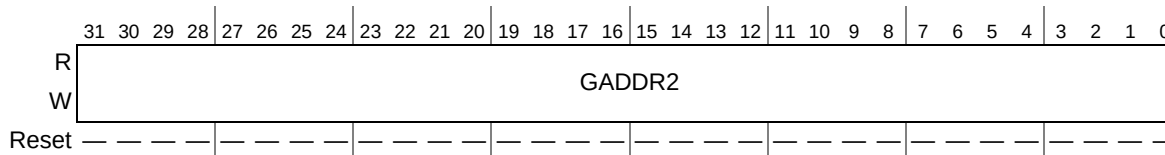
Figure 17-18. Descriptor Group Lower Address Register (GALR)
