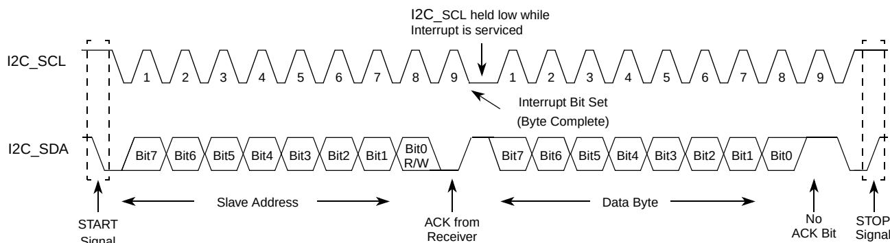
Figure 24-8. Data Transfer
