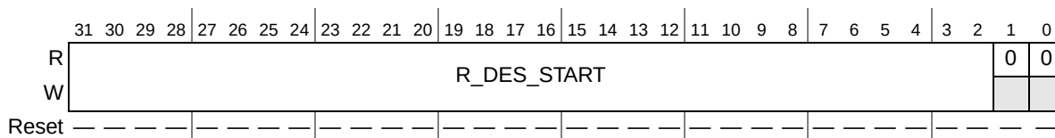
Figure 17-22. Ethernet Receive Descriptor Ring Start Register (ERDSR)
