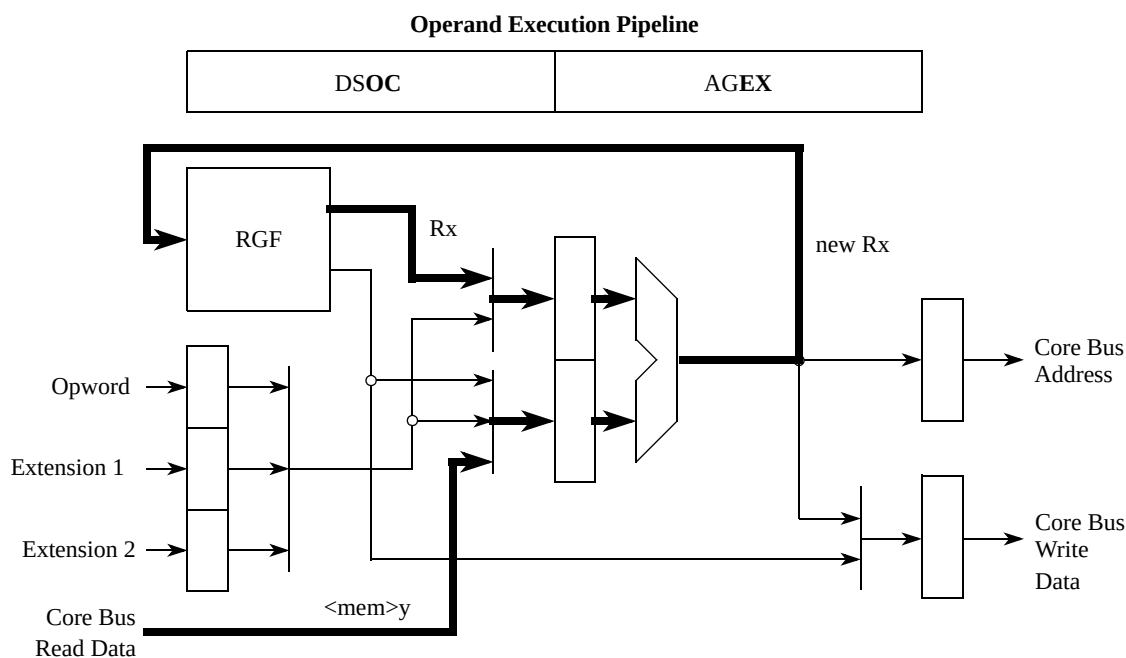
Figure 2-13. V2 OEP Embedded-Load Part 2
