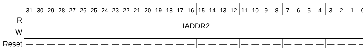
Figure 17-16. Descriptor Individual Lower Address Register (IALR)
