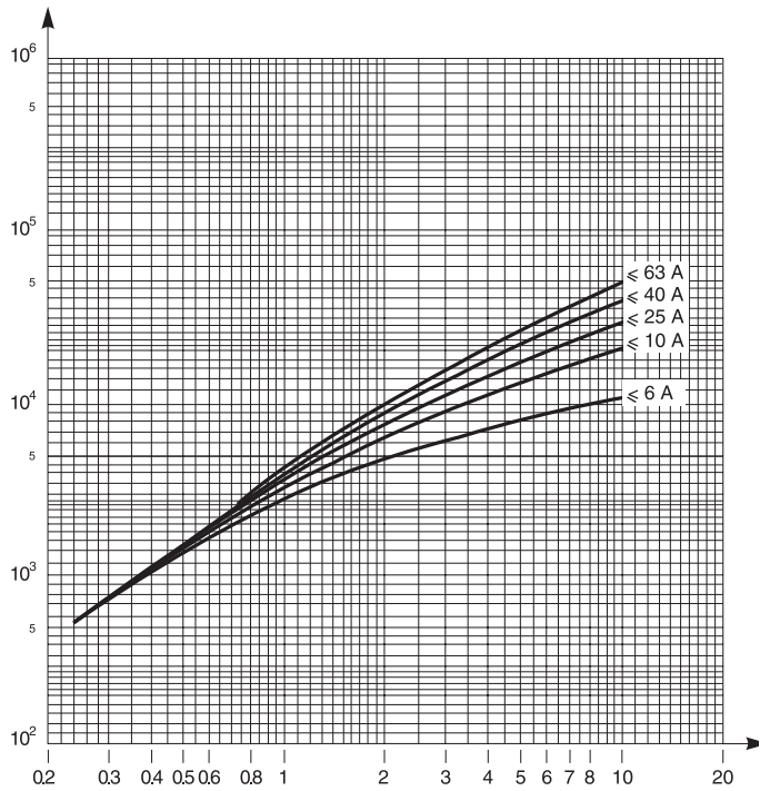
Figure 99: UL 1077 Recognized C60 2P, 3P, and 4P (480Y/277 Vac) Maximum Let-Through I²t Current
