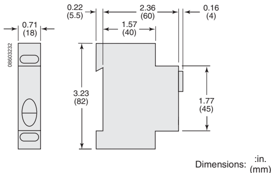
Figure 75: CH Hour Counter
