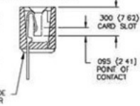
SINGLE ROW CONTACTS
