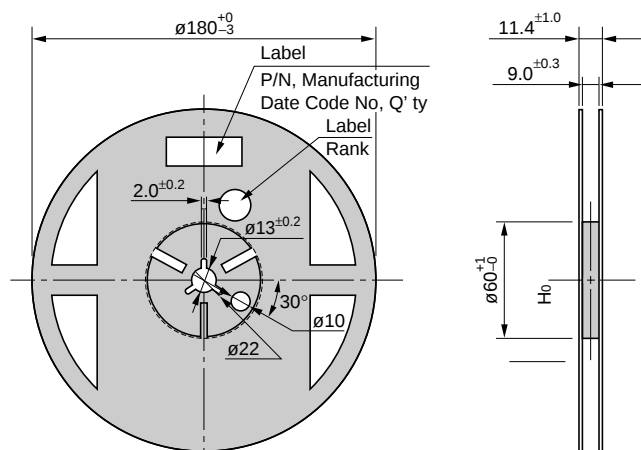
Reel specifications
