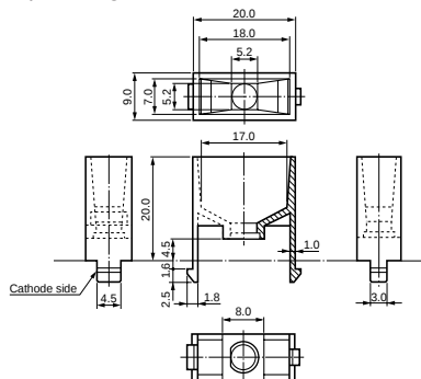
SEL9104 Lamp Casing
