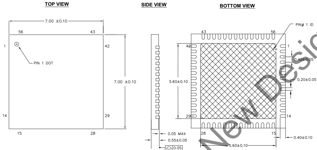
Figure 5. 56-Pin QFN 7 mm × 7 mm × 0.6 mm
