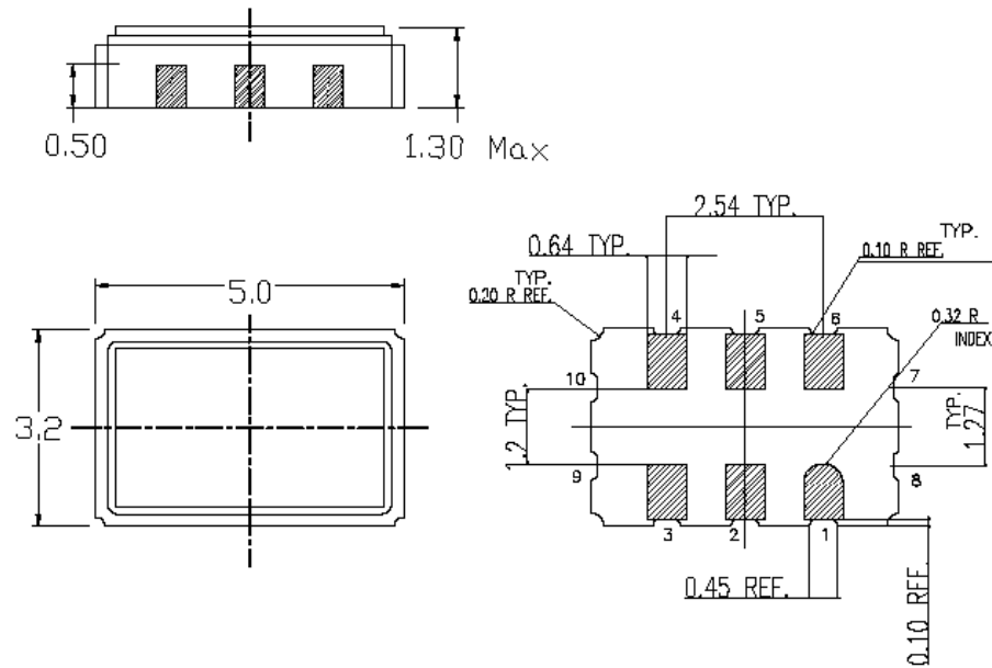
Figure 5. 6-Pin 3.2 × 5.0 mm Ceramic LCC
