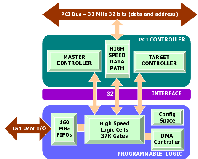
FIGURE 1. QL5032 Diagram
