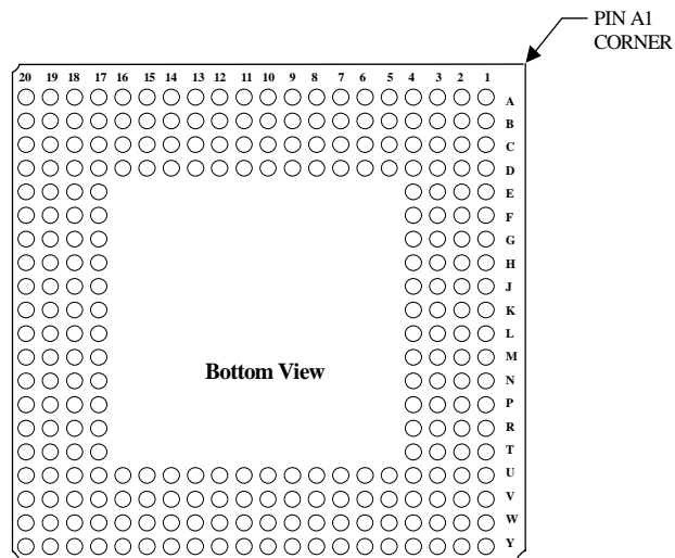
FIGURE 7. 256-pin PBGA
