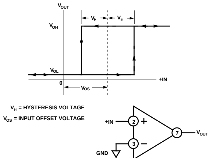
Figure 14. Hysteresis Definitions (N, Q Package Pinout)
