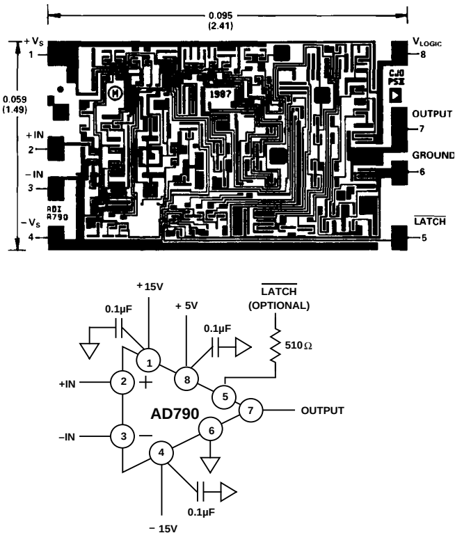
Figure 1. Basic Dual Supply Configuration (N, Q Package Pinout)
