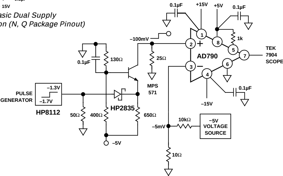
Figure 3. Response Time Test Circuit (N, Q Package Pinout)
