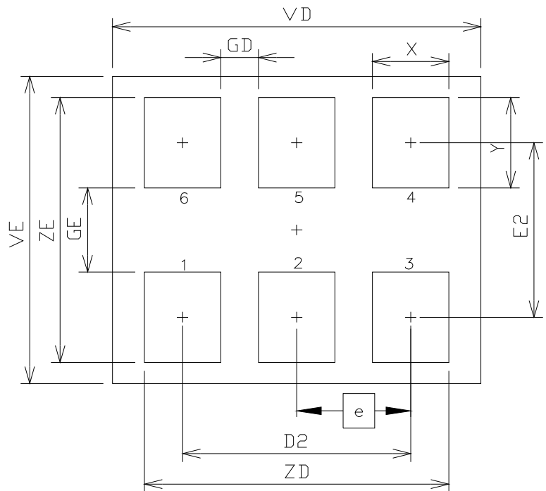
Figure 3. Si552 PCB Land Pattern
