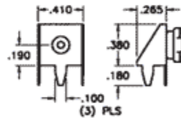
Mounting Detail
