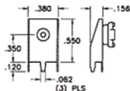
Mounting Detail
