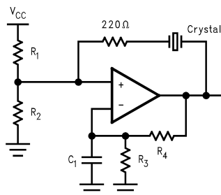
Figure 39. Crystal Oscillator
