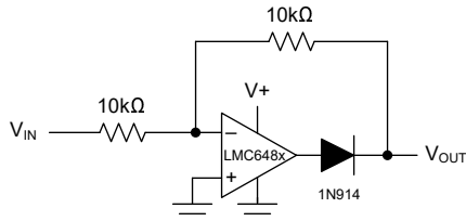
Figure 7-19. Full-Wave Rectifier With Input Current Protection ( R_i )
