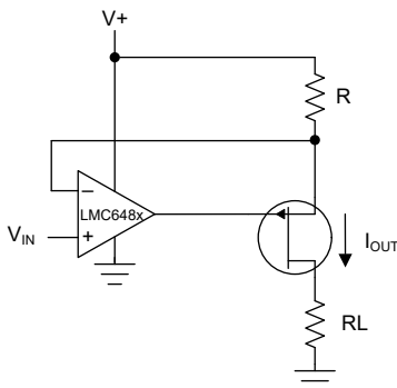
Figure 7-21. Large Compliance Range Current Source
