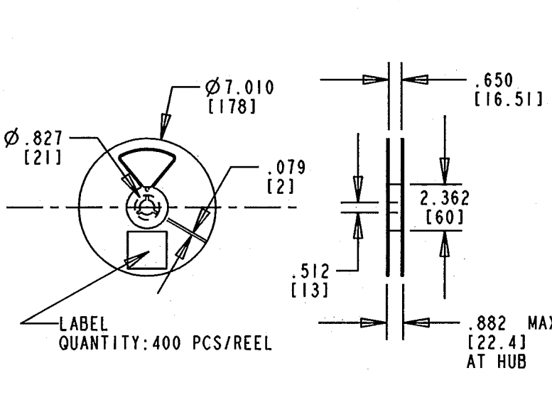
7 INCH DIA. REEL SPECIFICATIONS
