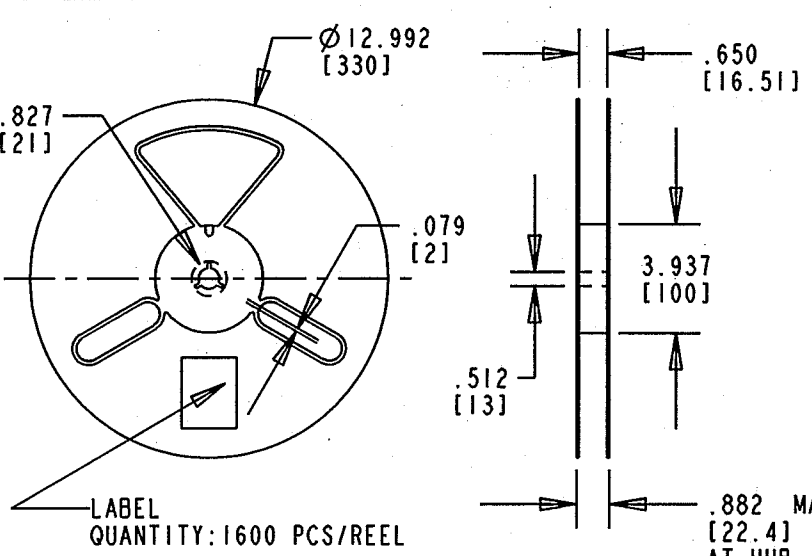
13 INCH DIA. REEL SPECIFICATIONS
