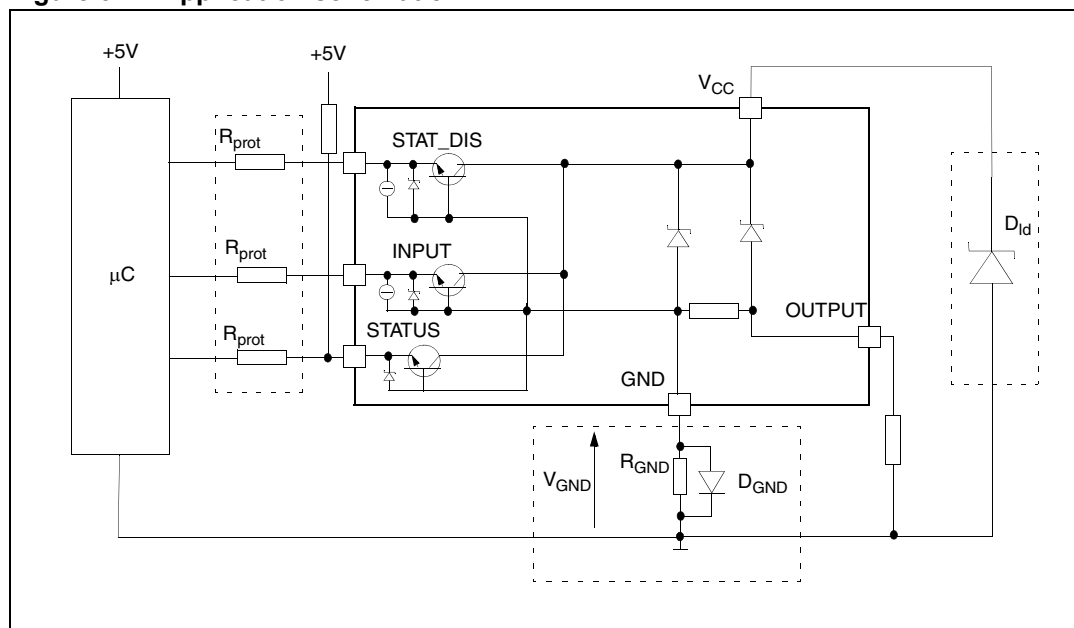
Figure 32. Application schematic
