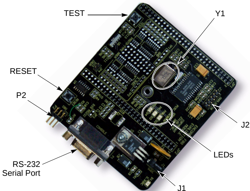
Figure 14. Z8 Encore!® 8K/4K Evaluation Board
