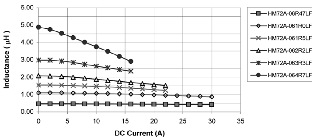
Inductance vs. Current Characteristics
