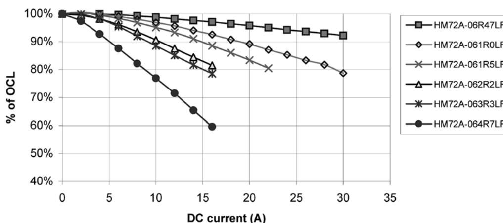
Inductance Rolloff vs. Current Characteristics
