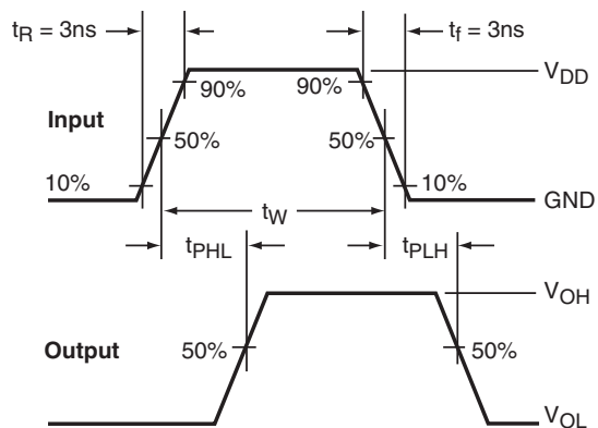
Figure 3. AC Waveforms
