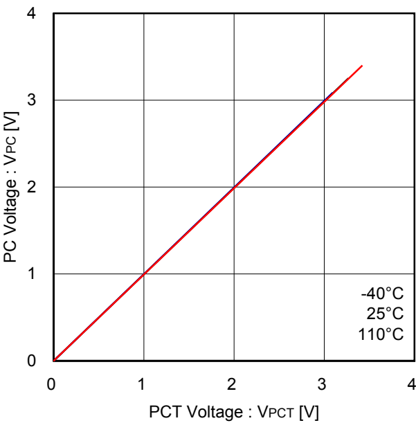
Figure 33. PCT - PC Linearity (R PCT =R PC =100kΩ)
