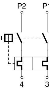
Undervoltage release with additional contact
