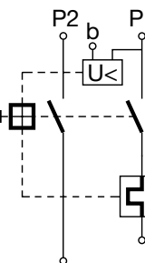
Mechanical lock-out latch
