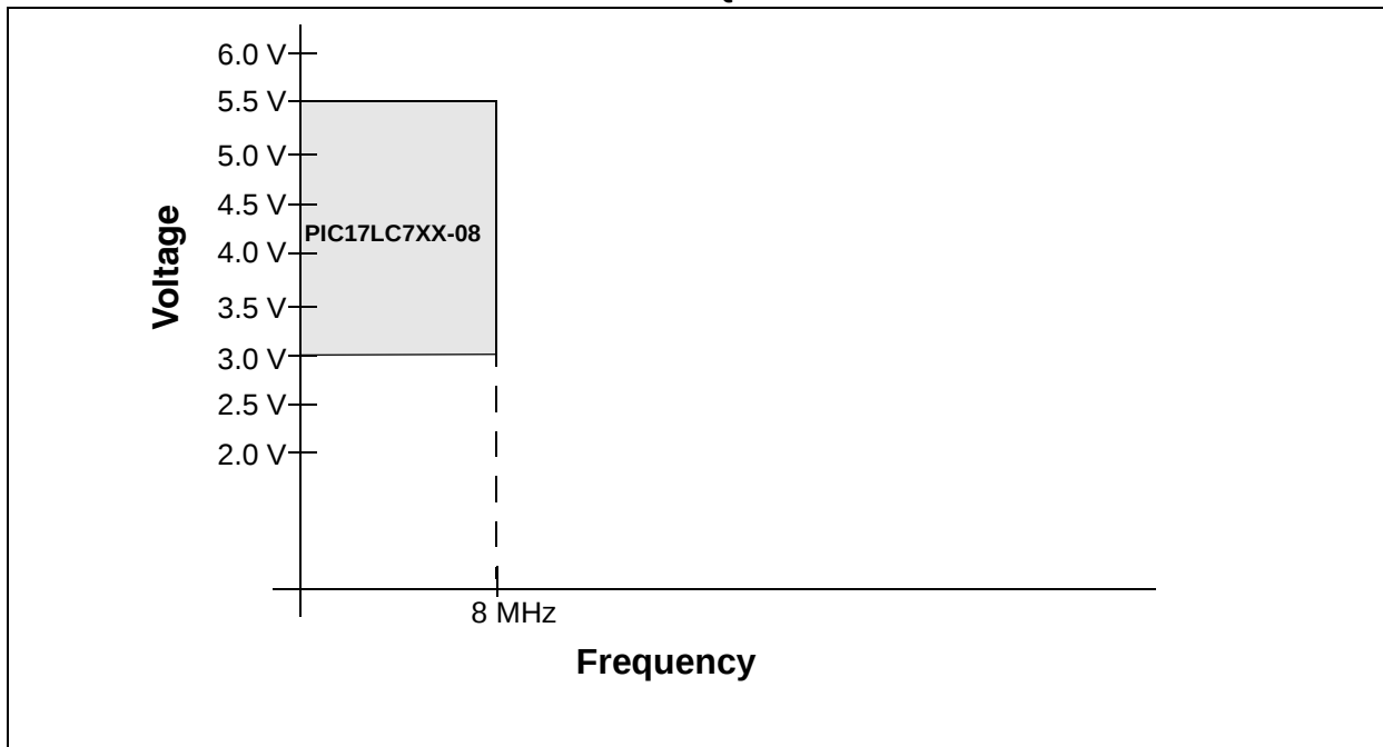
FIGURE 20-3: PIC17LC7XX-08 VOLTAGE-FREQUENCY GRAPH
