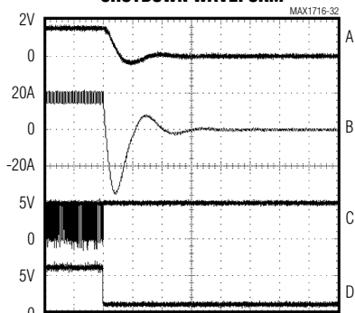
SHUTDOWN WAVEFORM
