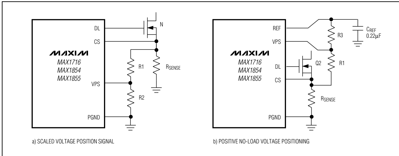
Figure 6. Voltage-Positioning Configurations
