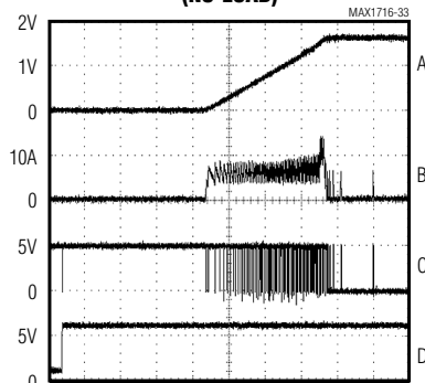
STARTUP WAVEFORM (NO-LOAD)
