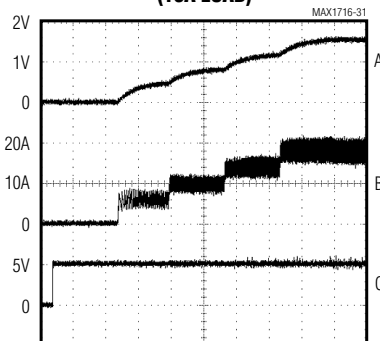
STARTUP WAVEFORM (18A LOAD)
