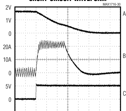
SHORT-CIRCUIT WAVEFORM
