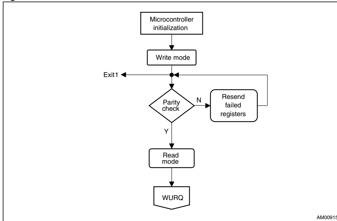
Figure 24. Device initialization
