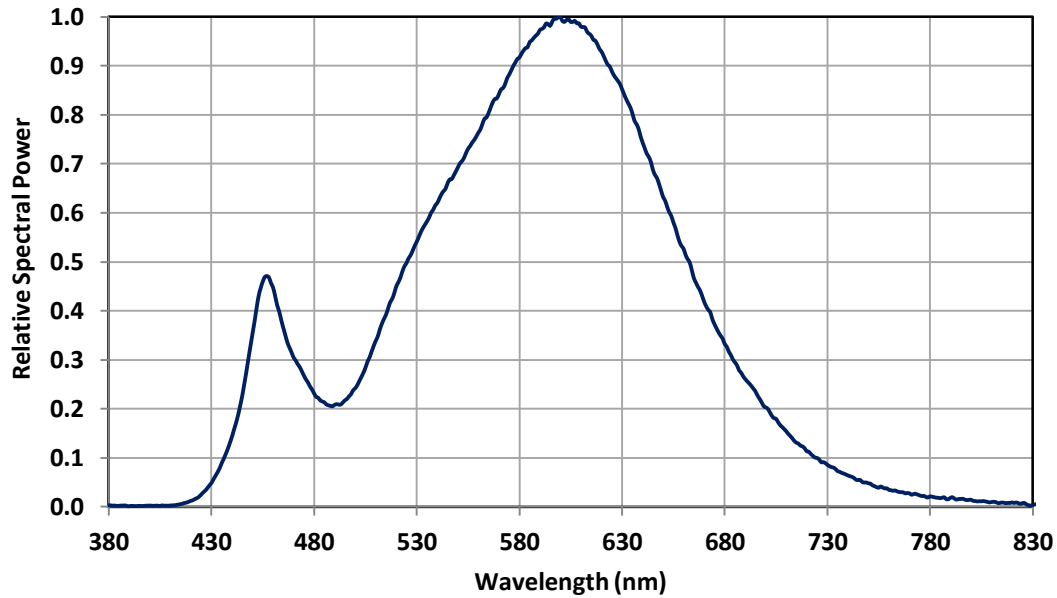
Figure 5: Typical relative spectral power vs. wavelength @ T_c = 25^\circ\text{C} , 3000K CRI 80
