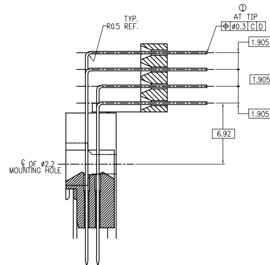
SECTION "Z"-Z" (5/1)
