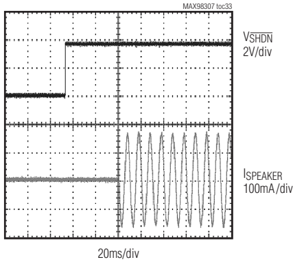
STARTUP RESPONSE
