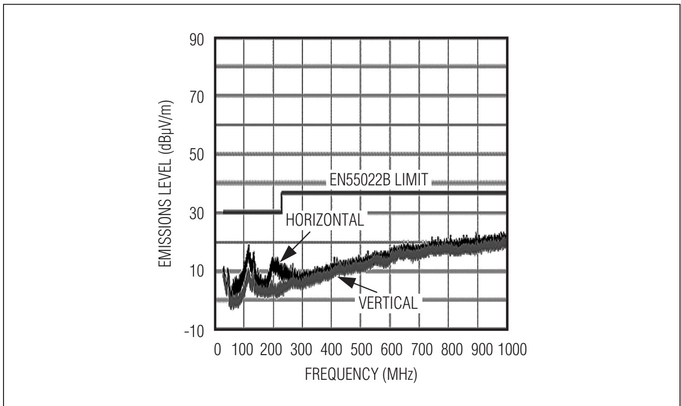
Figure 3. EMI Performance with V_{PVD} = 5V, 12in of Speaker Cable, No Output Filter
