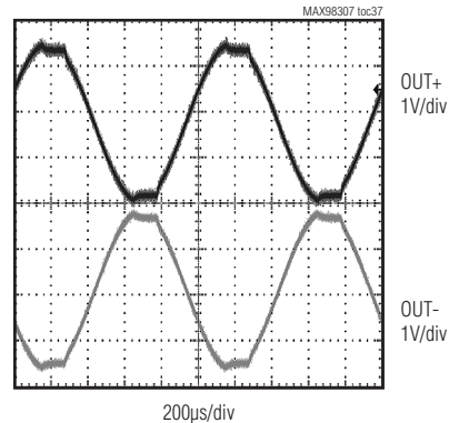
CLIPPING WAVEFORM 10% THD+N
