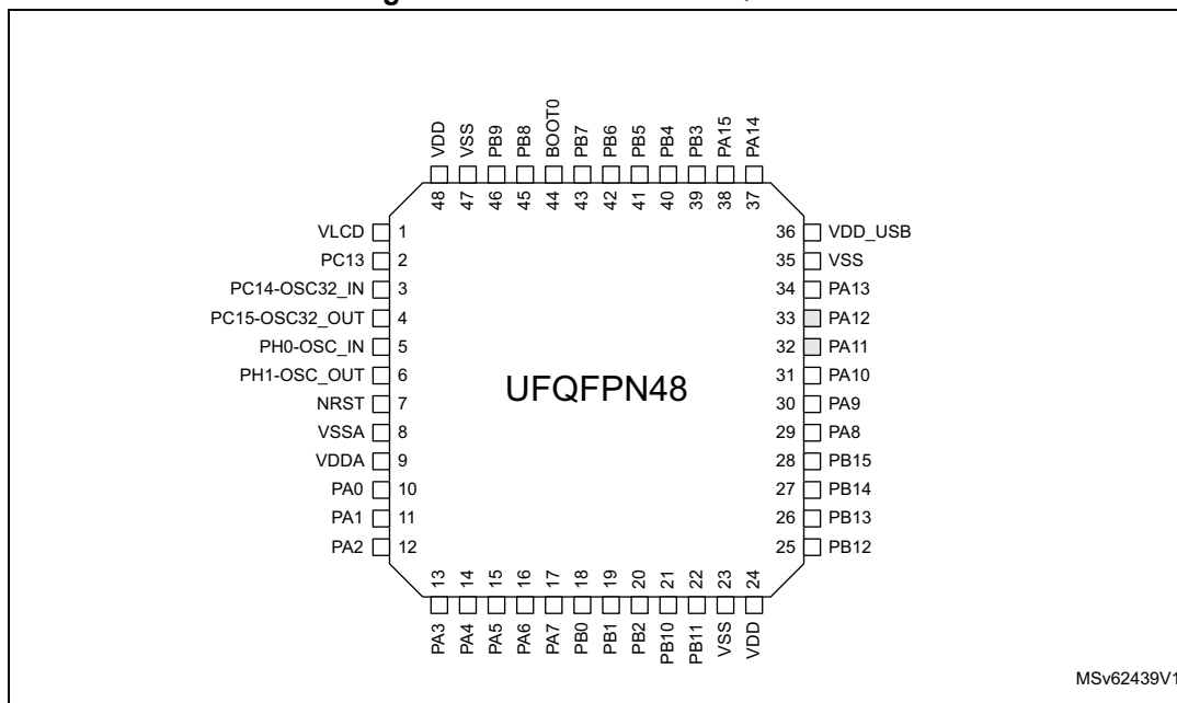
Figure 8. STM32L083xx UFQFPN48
