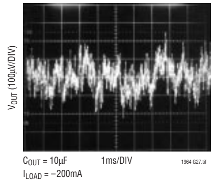
LT1964-5, 10Hz to 100kHz Output Noise, C_BY = 100pF
