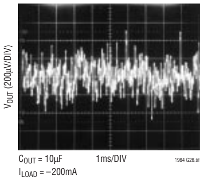
LT1964-5, 10Hz to 100kHz Output Noise, C_BY = 0
