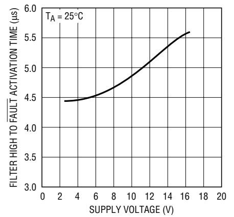
FILTER High to \overline{FAULT} Activation Time vs Supply Voltage
