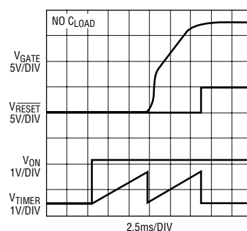
Power-Up Sequence
