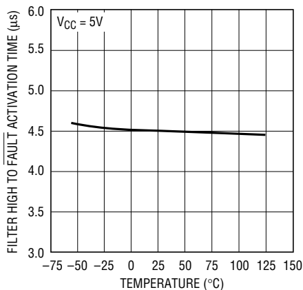
FILTER High to \overline{FAULT} Activation Time vs Temperature
