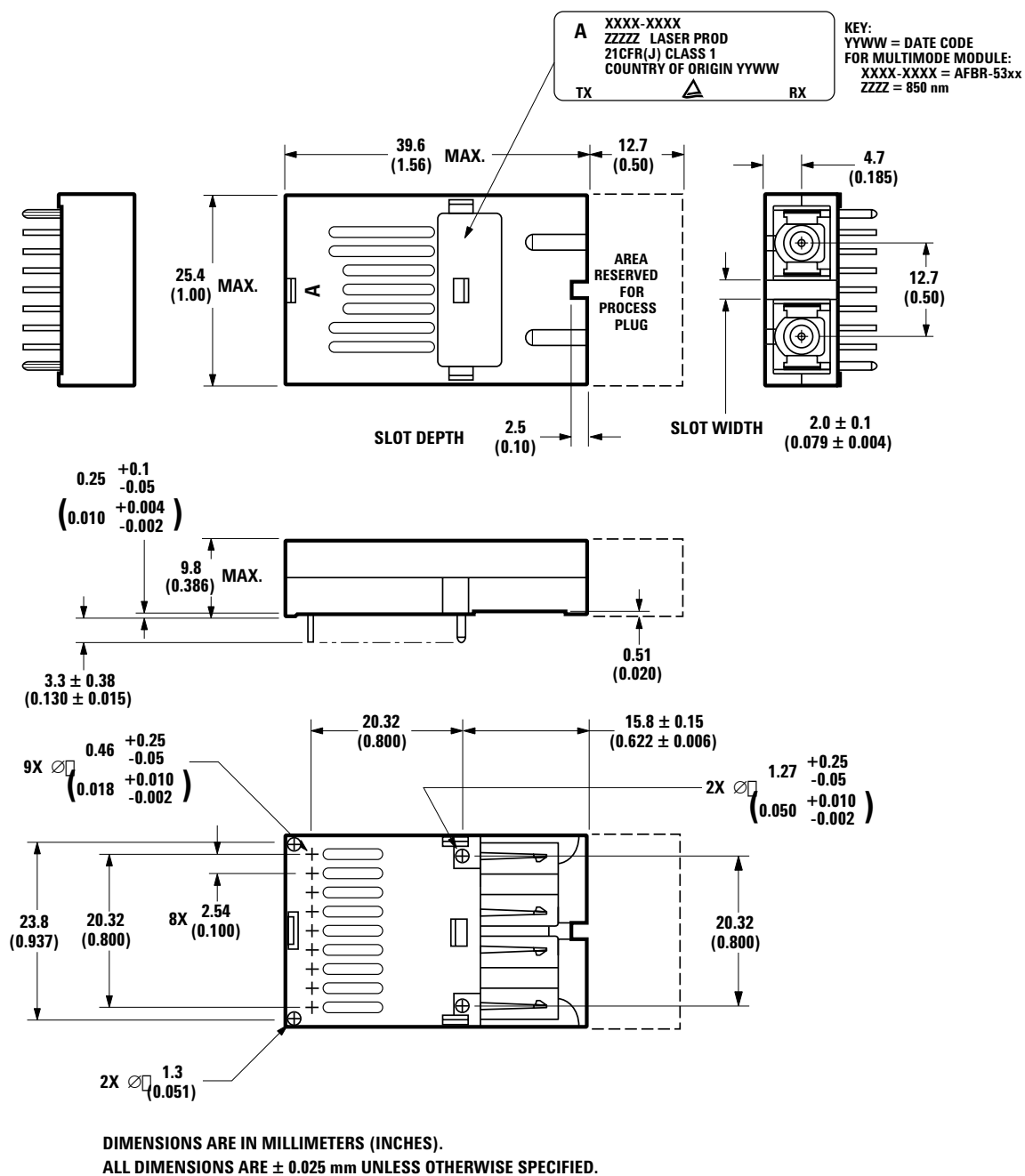
Figure 5. Package Outline Drawing for AFBR-53DSZ.
