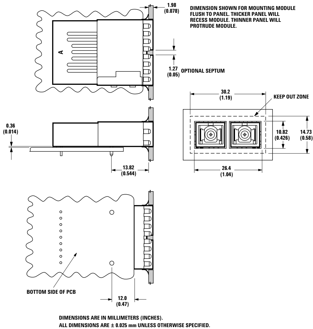
Figure 9. Suggested Module Positioning and Panel Cut-out for AFBR-53D5FZ.
