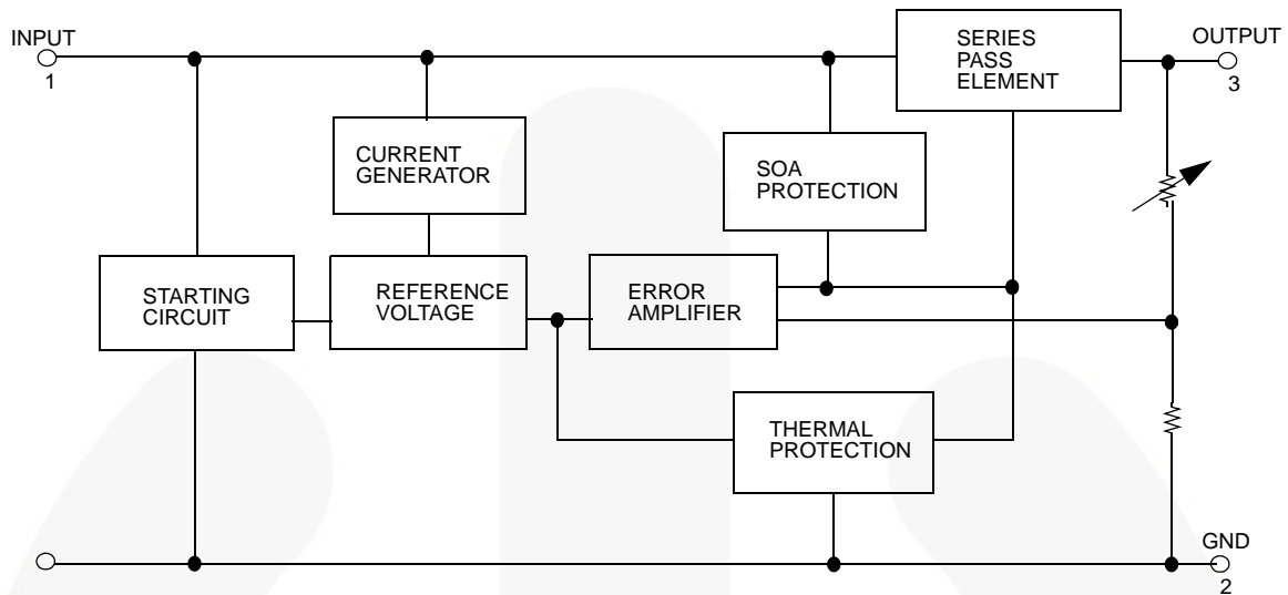
Figure 1. Block Diagram
