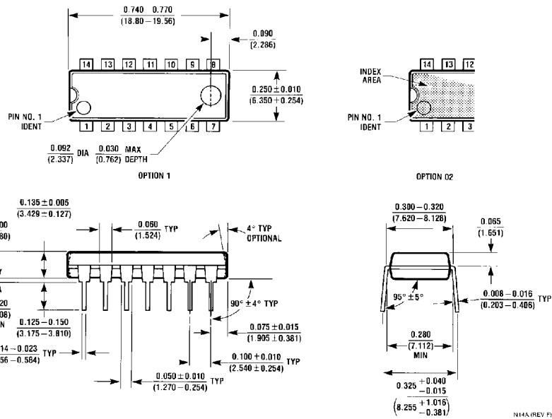
Molded Dual-In-Line Package (N) Order Number DM74ALS03BN Package Number N14A
