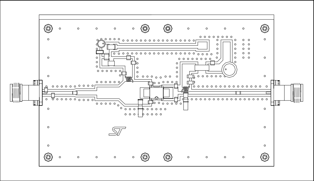
Figure 16. Test circuit
