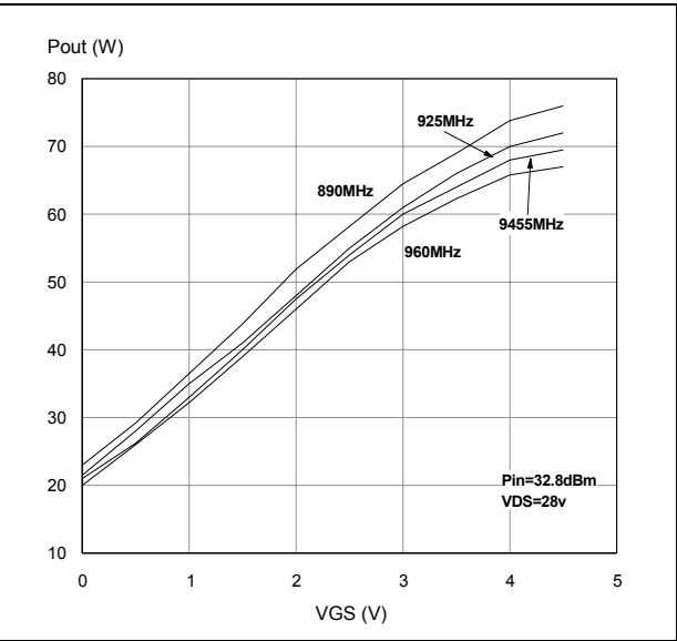
Figure 14. Output power vs gate-source voltage
