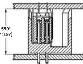
Figure 4 Double-Row, Two-Piece Receptacle and Two-Piece Shrouded Header *Mod II Shrouded Header Height is .440 [11.18] for a total stack height of .440 [11.18]
