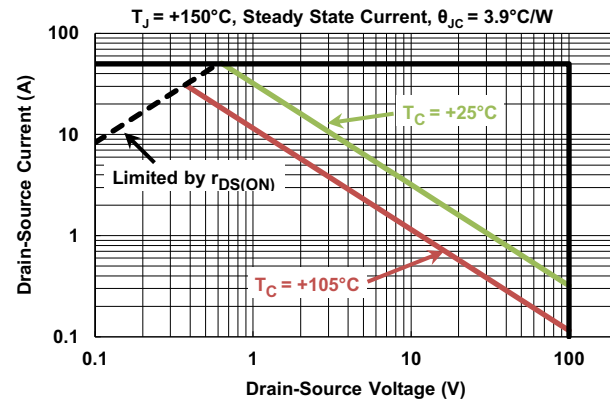
Figure 16. Safe Operating Area (Derated)
