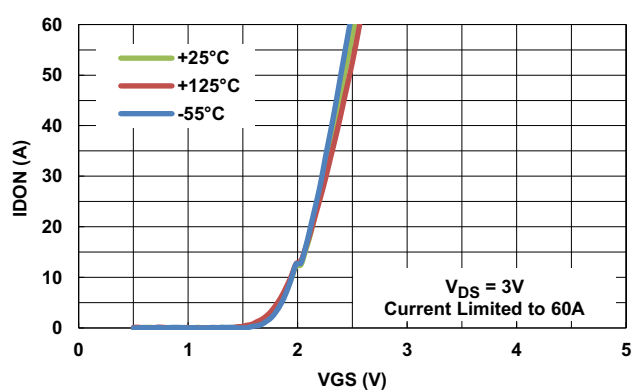
Figure 6. Transfer Characteristics
