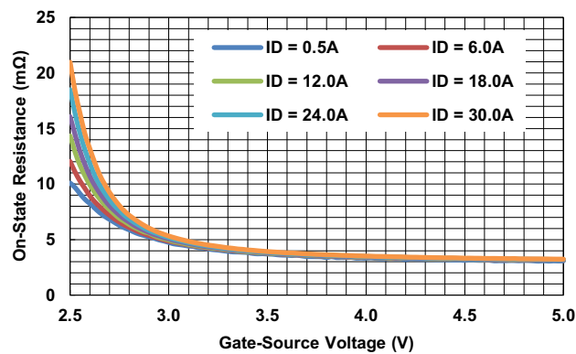
Figure 9. On-State Resistance ( -55^{\circ}C )
