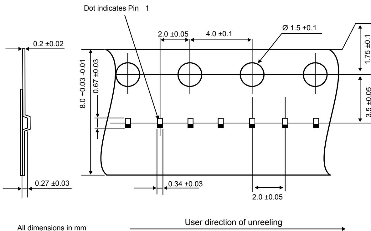
Figure 9. Tape and reel specification (in mm)
