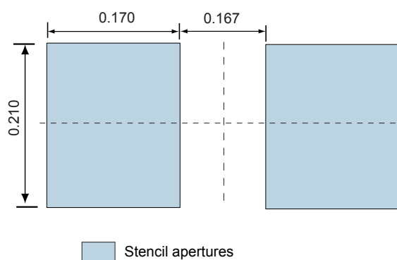
Figure 11. Recommended stencil window position in mm
