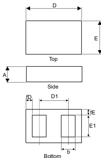
Figure 8. 0201 WLCSP package outline
