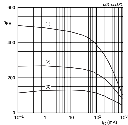
V_{CE} = -2\text{ V} (1) T_{amb} = 150\text{ }^{\circ}\text{C} (2) T_{amb} = 25\text{ }^{\circ}\text{C} (3) T_{amb} = -55\text{ }^{\circ}\text{C}
