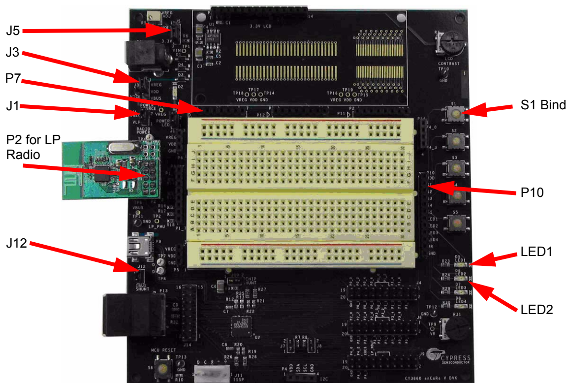
Figure 5-1. WUSB_Example Bridge
