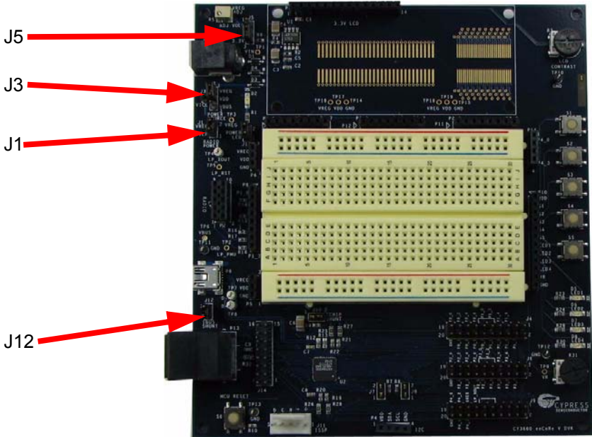
Figure 4-1. ISOC_Example
