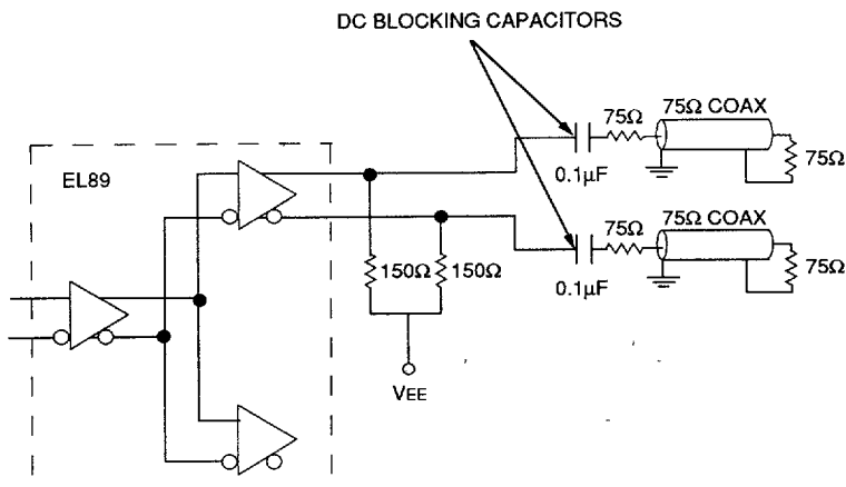
Figure 1. Termination Configuration
