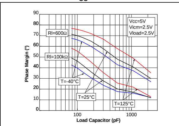
Figure 11. Phase margin vs. load capacitor at V_{CC} = 5\text{ V}
