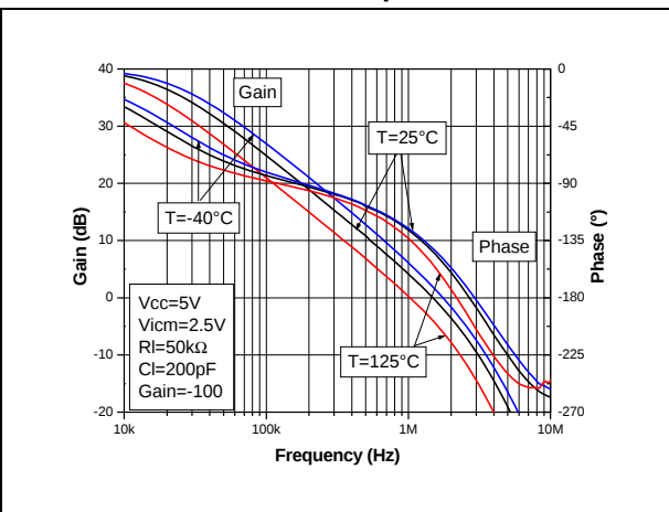
Figure 9. Voltage gain and phase with C_I = 200\text{ pF}
