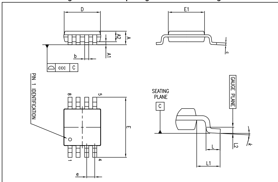
Figure 30. MiniSO8 package mechanical drawing
