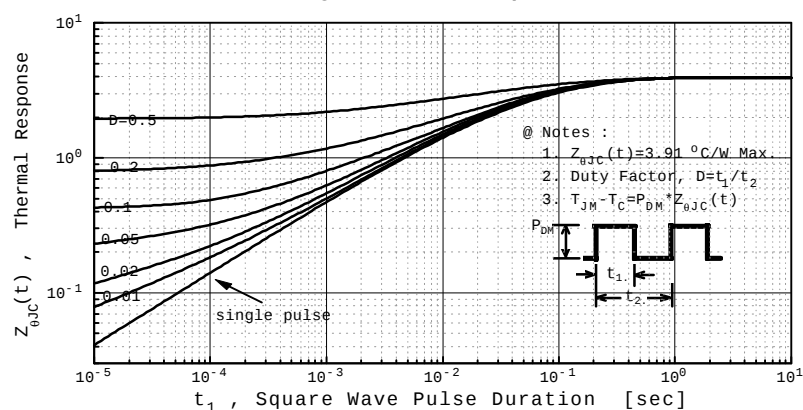
Fig 11. Thermal Response
